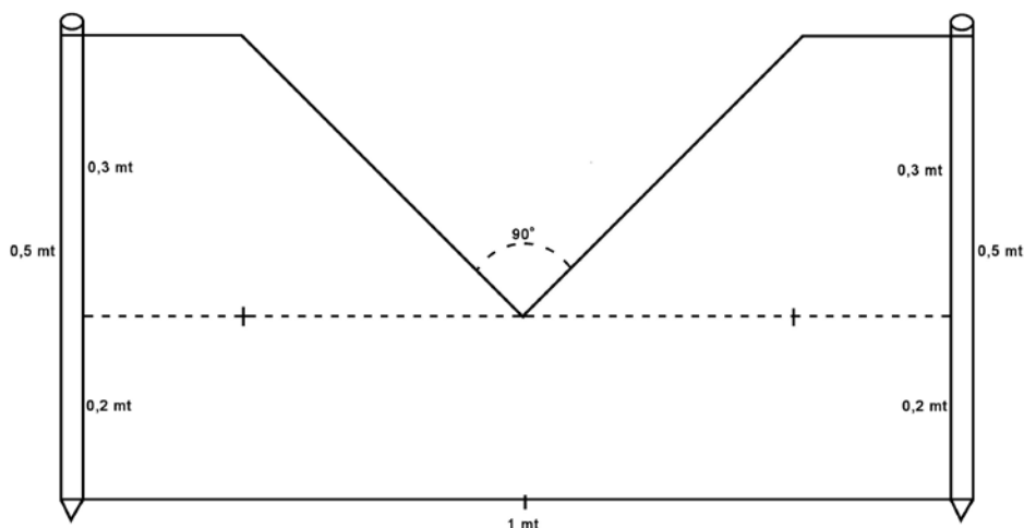
Vertedouro triangular
